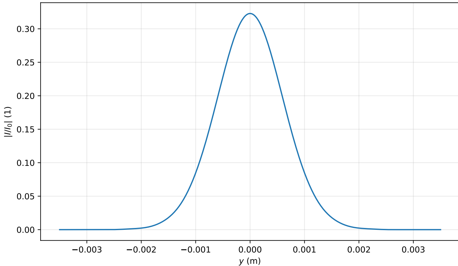
Intensity profile I(x = 0, y, z = 3.344)/I_0 , P_{in}=0.2P_{cr} , artificial time
